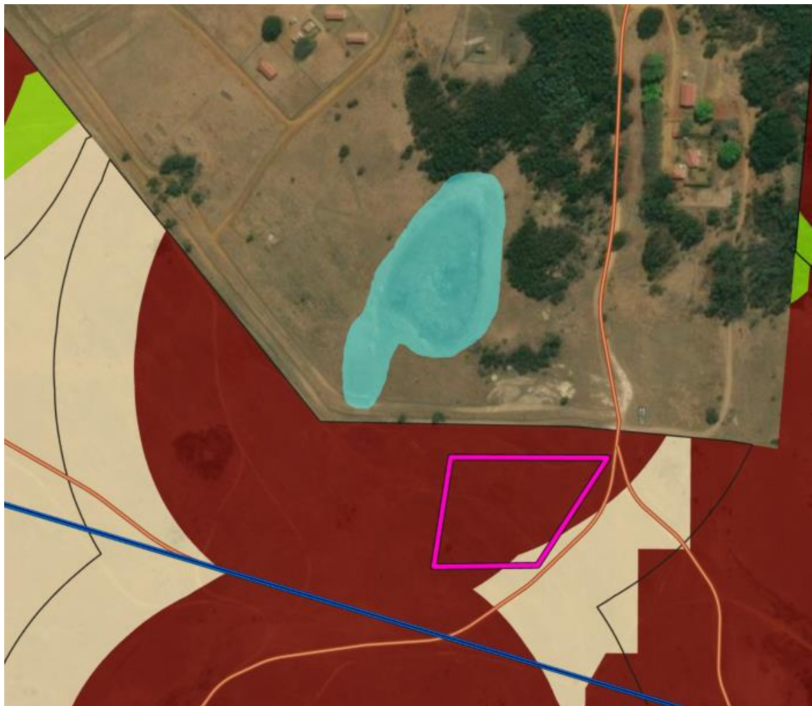
FIGURE 10-1 : O&M BUILDING WITHIN A NO-GO BUFFER (DARK RED) MUST BE RELOCATED OR ADDITIONAL MITIGATION MEASURES APPLIED
