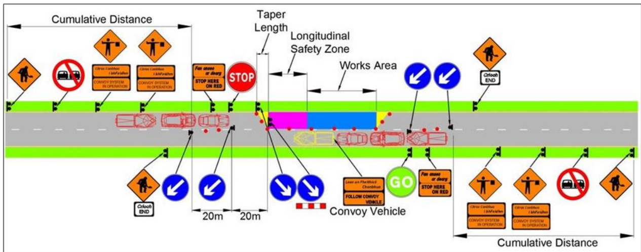
FIGURE 17.1 STOP-GO OPERATION (SOURCE: TEMPORARY TRAFFIC MANAGEMENT DESIGN GUIDANCE)
