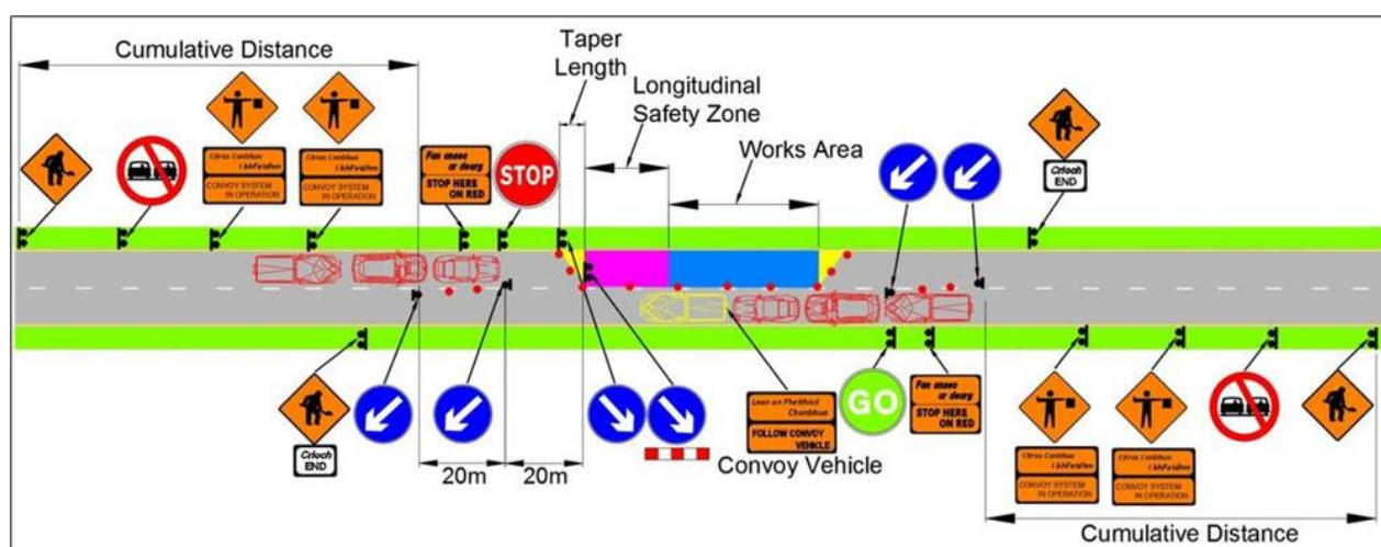
FIGURE 16-1 STOP-GO OPERATION (SOURCE: TEMPORARY TRAFFIC MANAGEMENT DESIGN GUIDANCE)
