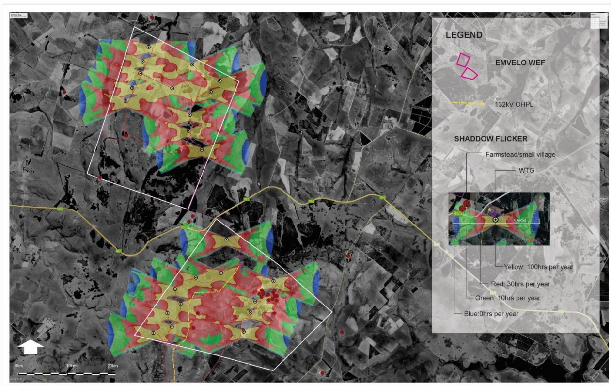
FIGURE 10-2 FLICKER ANALYSIS
