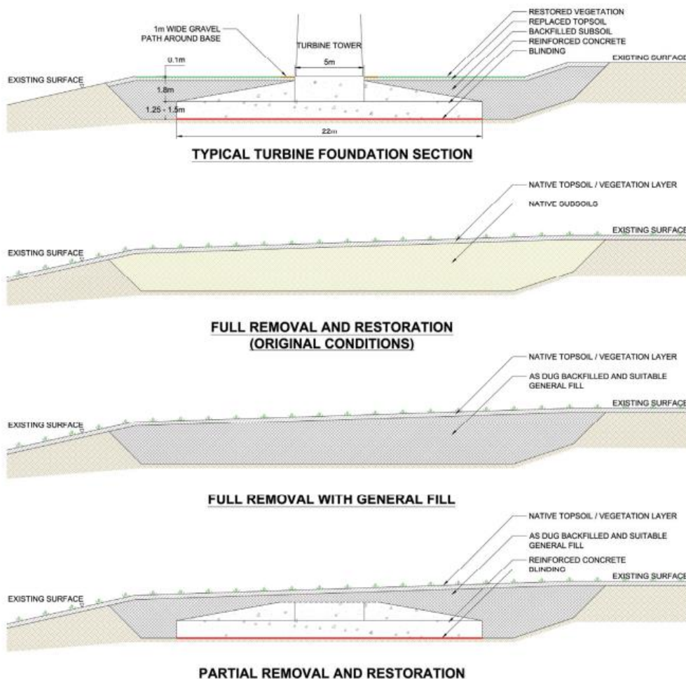
FIGURE 11.1 TURBINE FOUNDATION DECOMMISSIONING ALTERNATIVES
